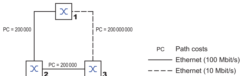
Figure 7: Path costs
