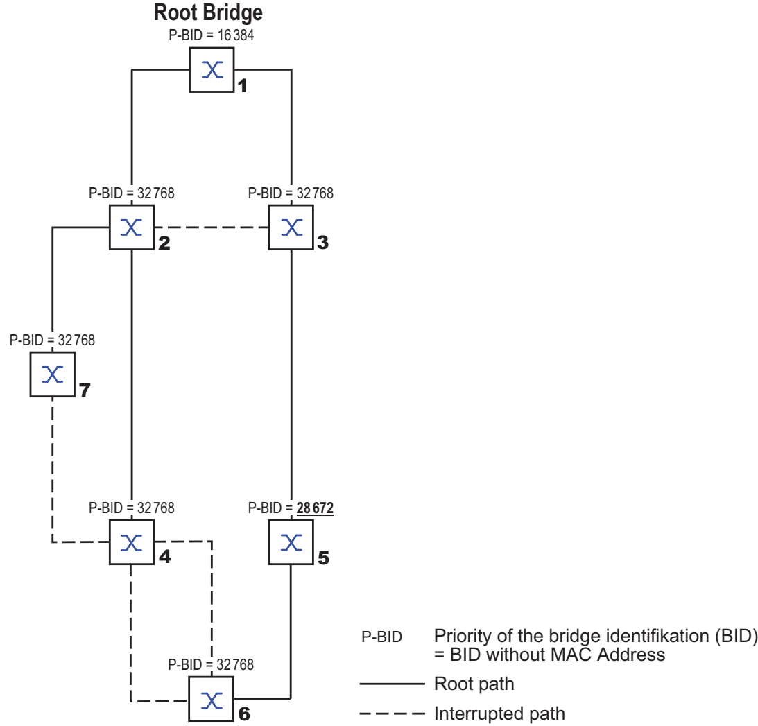
Figure 13: Example of manipulating the root path
