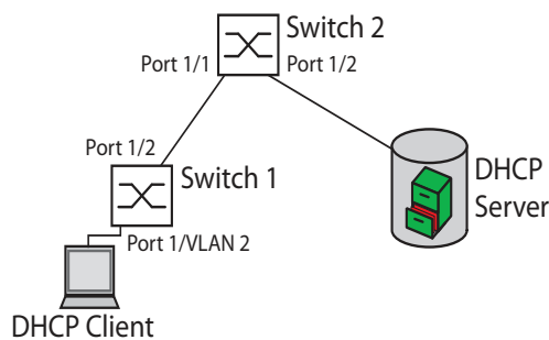
Figure 70: DHCP Layer 2 Example Network
