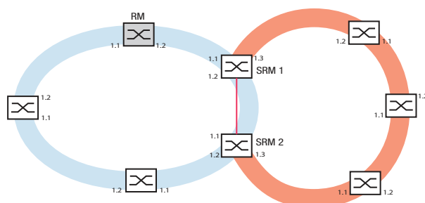
Figure 51: Example of a subring structure blue ring = Main ring orange ring = Subring red line = Redundant link of Subring SRM = Subring Manager RM = Ring Manager
