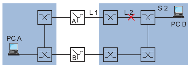
Figure 81: Monitoring a line with ping tracking
