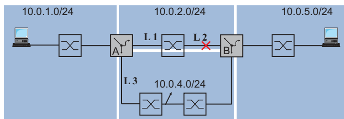
Figure 78: Example of static route tracking
