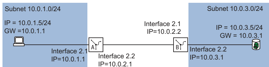
Figure 93: Example of the configuration of RIP
