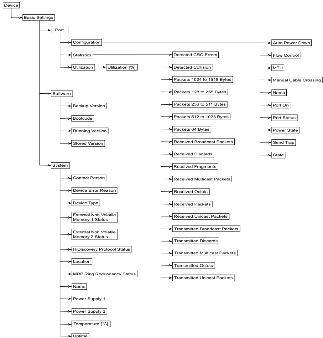
Figure 113: OPC UA information model
