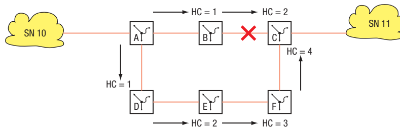
Figure 92: Hop count
