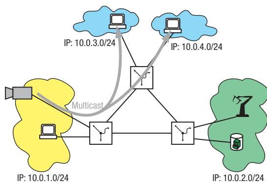
Figure 101: Example of a multicast application
