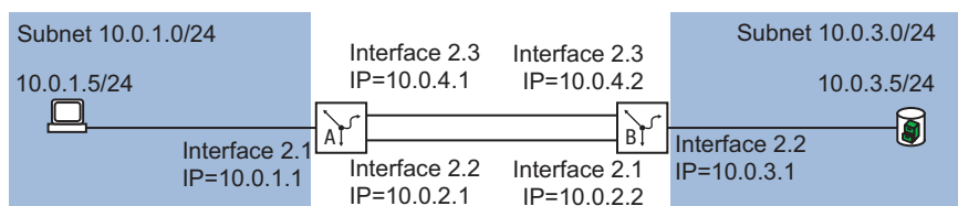
Figure 77: Redundant static route
