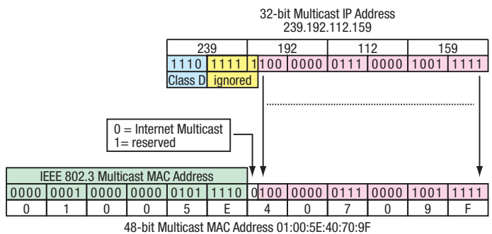
Figure 102: Conversion of the IP address to the MAC address
