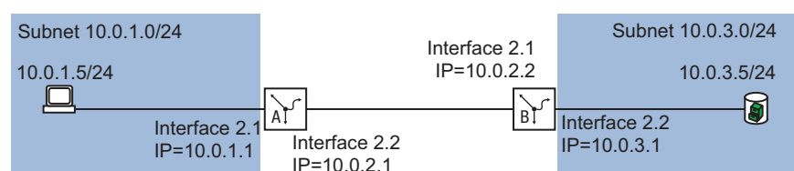
Figure 76: Static Routing
