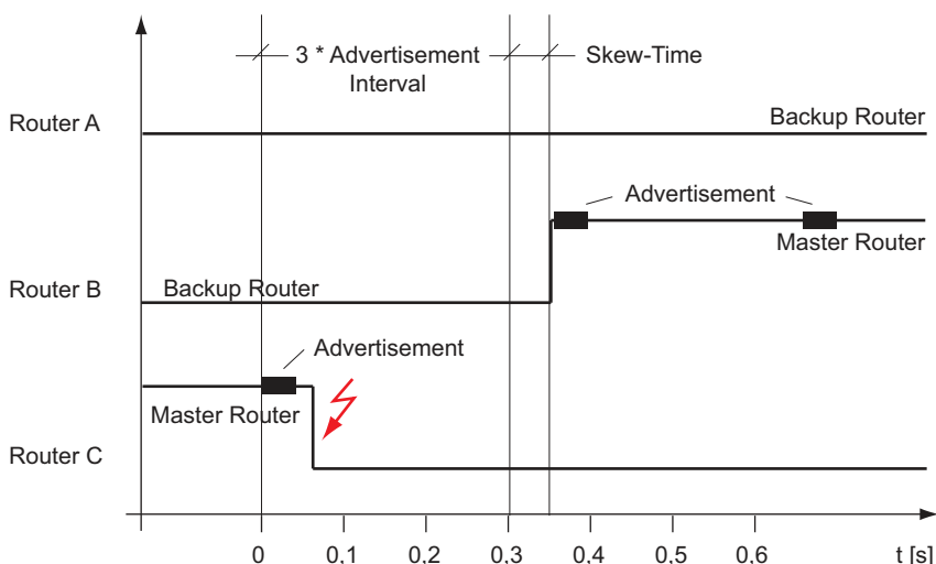
Figure 87: Master router <-> backup router failover times according to HiVRRP VRRP priority router A = 64 VRRP priority router B = 128 VRRP priority router C = 254
