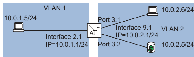
Figure 75: VLAN-based router interface
