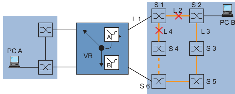
Figure 82: Monitoring the accessibility of a device in a redundant ring
