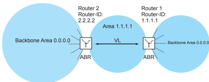
Figure 97: Expanding the backbone area using a virtual link (VL)
