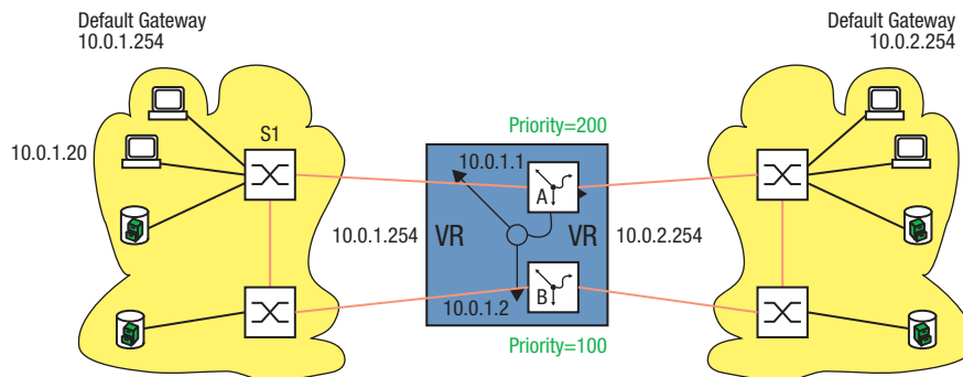
Figure 89: Virtual router with load sharing
