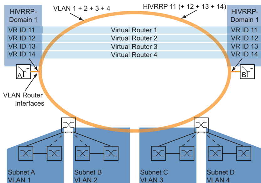
Figure 88: Example of how a HiVRRP domain is used
