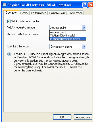
Figure 25: Changing the operating mode of the Access Points to 'managed'
