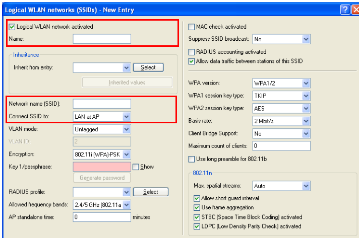
Figure 54: Logical WLAN networks for internal use
