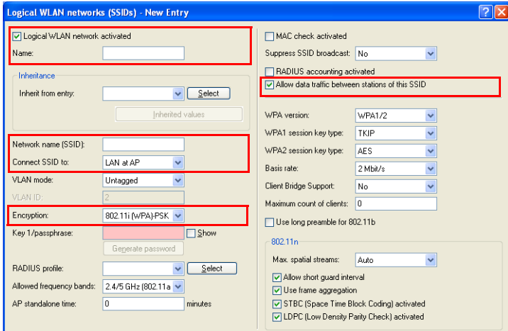
Figure 55: Logical WLAN networks for guest access
