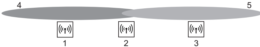
Figure 9: 1 - access point 1 (AP-1) 2 - access point 2 (AP-2) 3 - access point 3 (AP-3) 4 - network coverage area of access point 1 5 - network coverage area of access point 2
