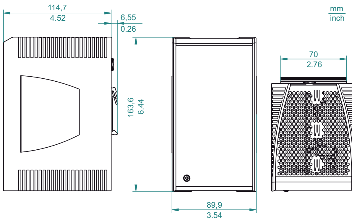
Figure 11: Dimensions of the device variants without WAN ports with operating characteristic value S. For the characteristic value, see “Device name and product code” on page 20.
