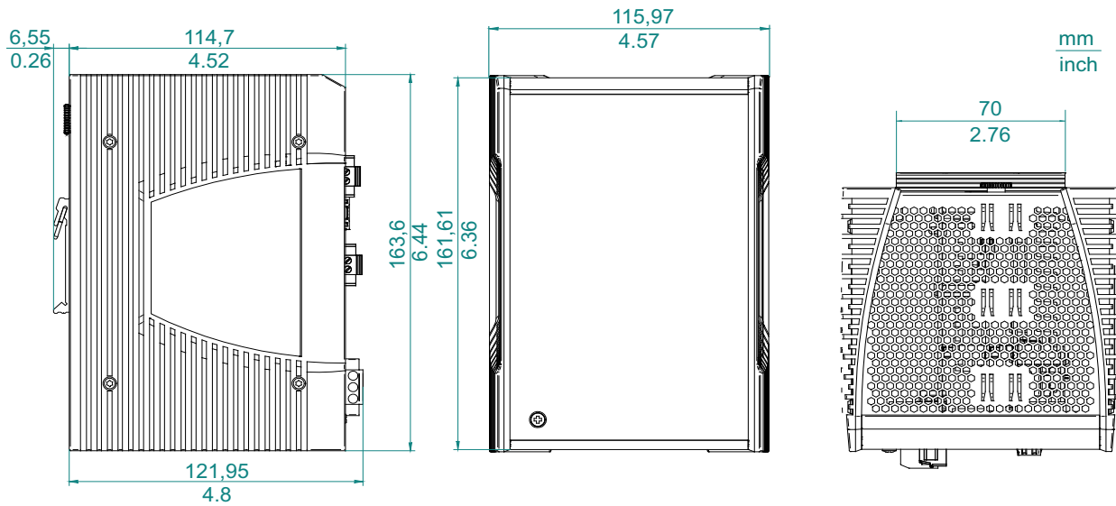
Figure 14: Dimensions of the device variants with WAN ports with operating characteristic value E and T. For the characteristic value, see “ Device name and product code ” on page 20.
