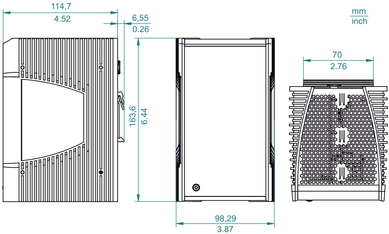
Figure 12: Dimensions of the device variants without WAN ports with operating characteristic value E and T. For the characteristic value, see “Device name and product code” on page 20.
