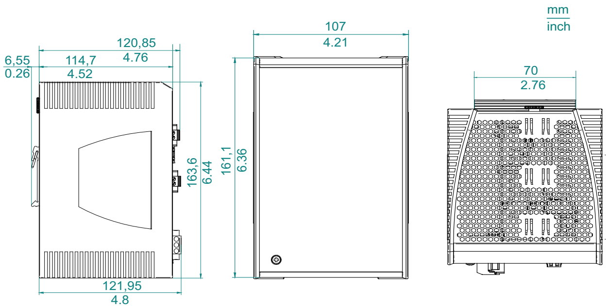
Figure 13: Dimensions of the device variants with WAN ports with operating characteristic value S. For the characteristic value, see “Device name and product code” on page 20.
