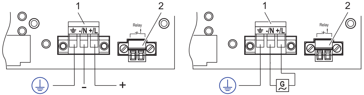
Figure 4: Power supply unit supply voltage characteristic value M (see on page 45 “General technical data”):
