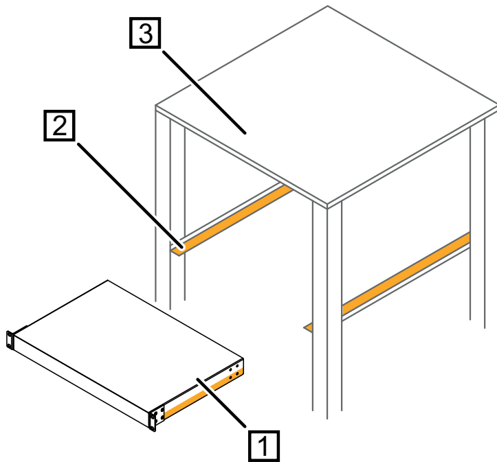
Figure 5: Assembly in a switch cabinet with sliding/mounting rails 1 - MACH1040 device 2 - sliding/mounting rail 3 - 19" switch cabinet
