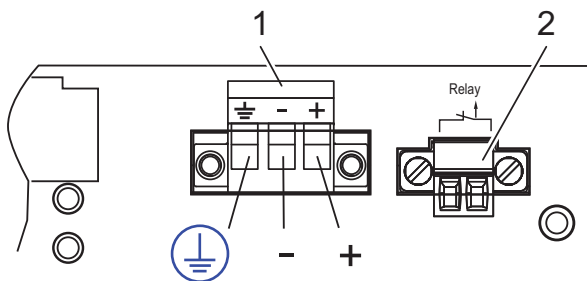
Figure 3: Power supply unit supply voltage characteristic value L, DC voltage (see on page 45 “General technical data” )
