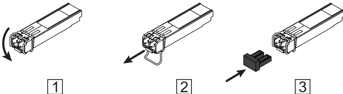
Figure 7: De-installing SFP transceivers: De-installation sequence
